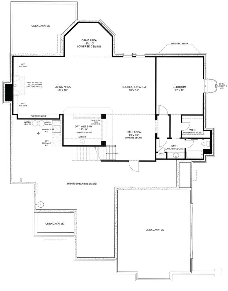
OPT. FINISHED LOWER LEVEL PLAN (INGRADE CONDITION)
