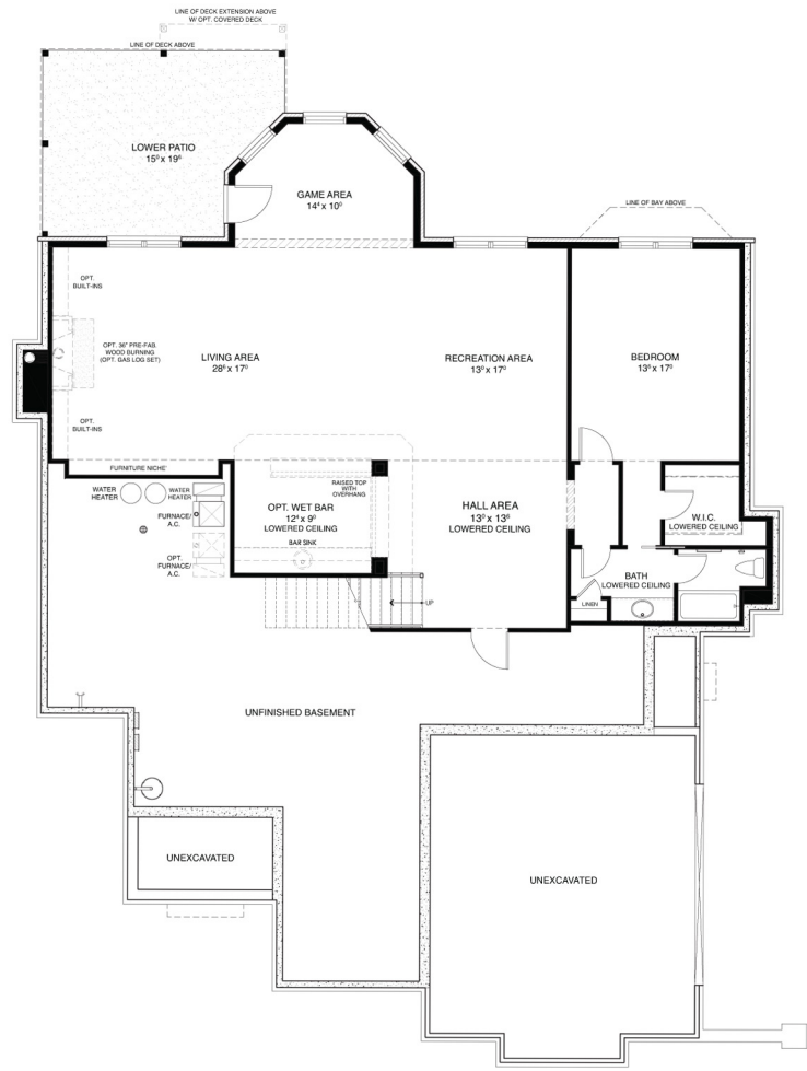
OPT. FINISHED LOWER LEVEL PLAN (WALKOUT CONDITION)
