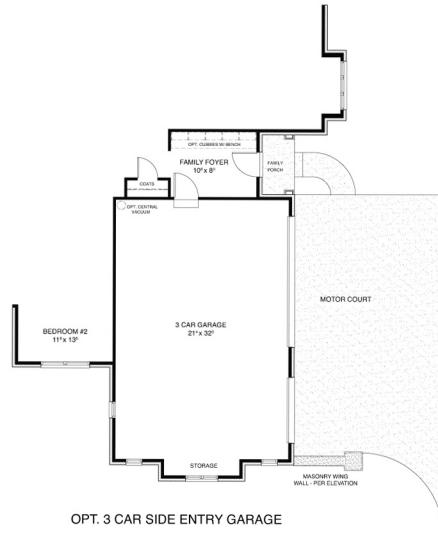
OPT. 3 CAR SIDE ENTRY GARAGE
