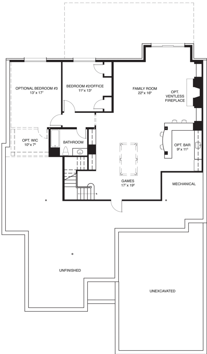
OPTIONAL FINISHED LOWER LEVEL
